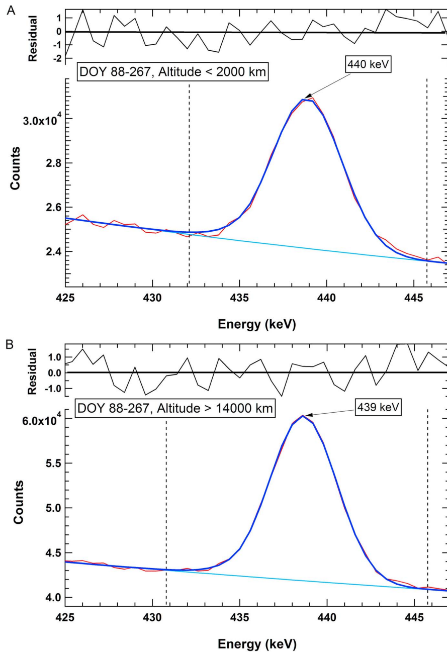
Figure 5. Fit of the Na(n,n'γ) 440 keV peak in (a) the low-altitude spectrum and (b) the high-altitude spectrum for the standard spectra accumulated between 29 March 2011 and 24 September 2011. The 439 keV label on the high-altitude fit corresponds to the ^{69\text{m}}\text{Zn} peak, though the energy resolution is not sufficient to distinguish between that and the 440 keV peak.
