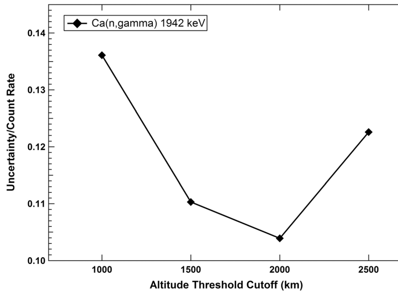
Figure 1. The variation of the uncertainty to peak count rates as a function of the low-altitude threshold for one example peak: \text{Ca}(n,\gamma) 1942 keV peak.
