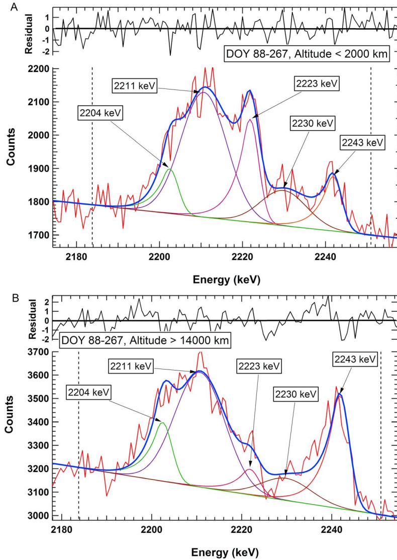
Figure 4. Fit of the S(n,n'γ) 2230 keV Doppler-broadened peak in (a) the low-altitude spectrum and (b) the high-altitude spectrum for the standard spectra accumulated between 29 March 2011 and 24 September 2011. The peaks in the spectra are Al(n,n'γ) at 2211 keV, H(n,γ) at 2223 keV, a peak from the decay of 238 U ( 214 Bi) at 2204 keV, and the single escape peak of 24 Na at 2243 keV.
